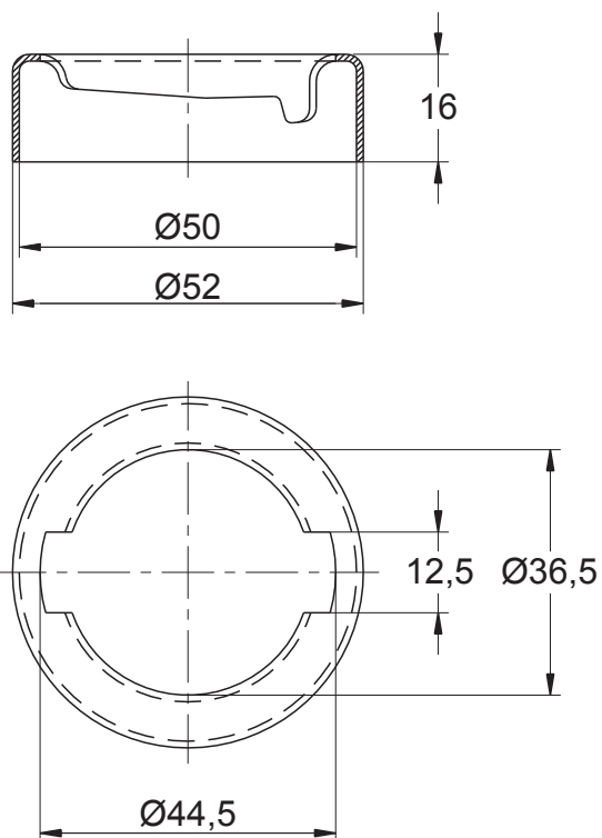
Embase DM014A
