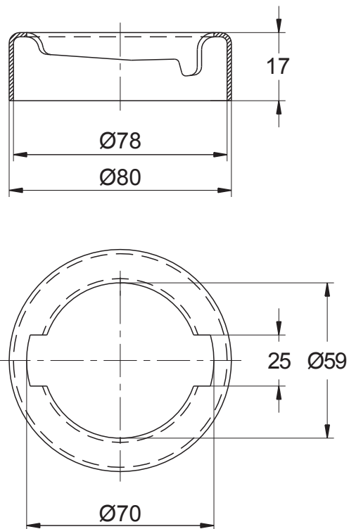
Embase DM016A
